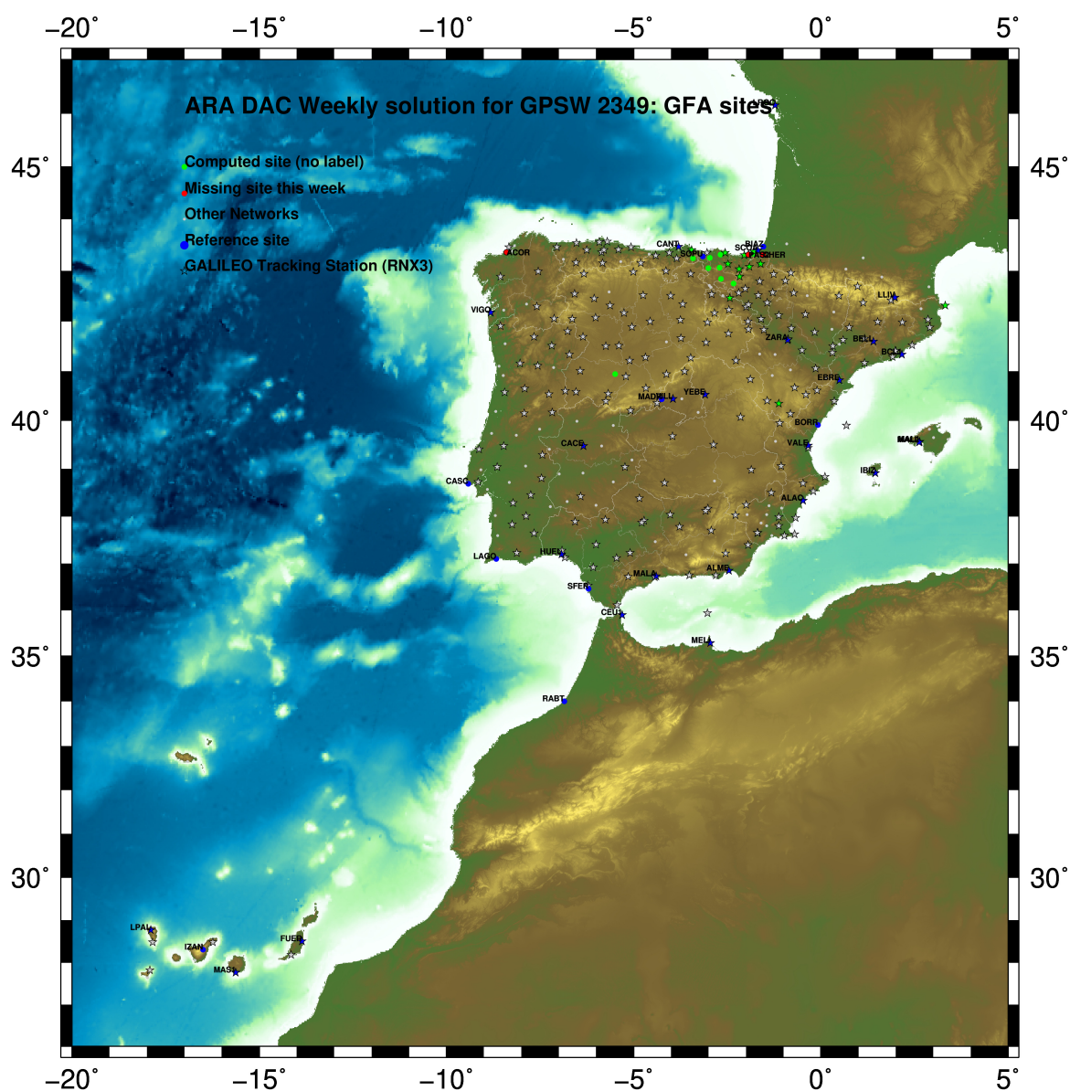
Fig.1: Computed Sites for GPS Week2349 (GFA)
