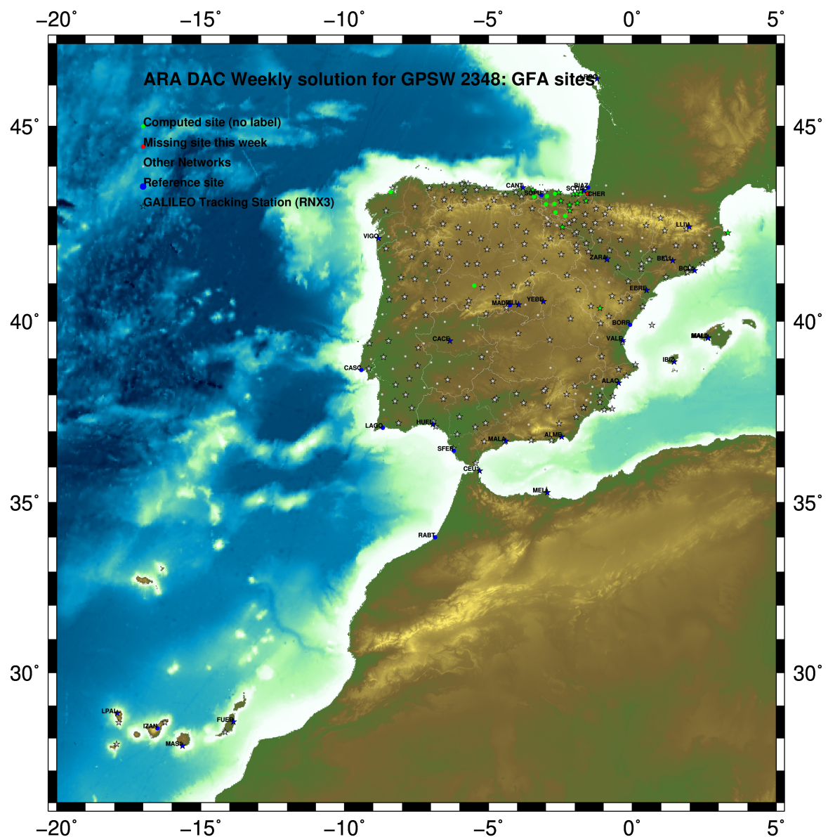
Fig.1: Computed Sites for GPS Week2348 (GFA)
