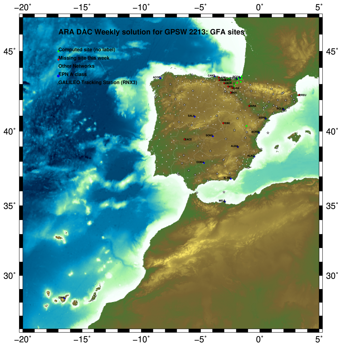
Fig.1: Computed Sites for GPS Week2213 (GFA)
