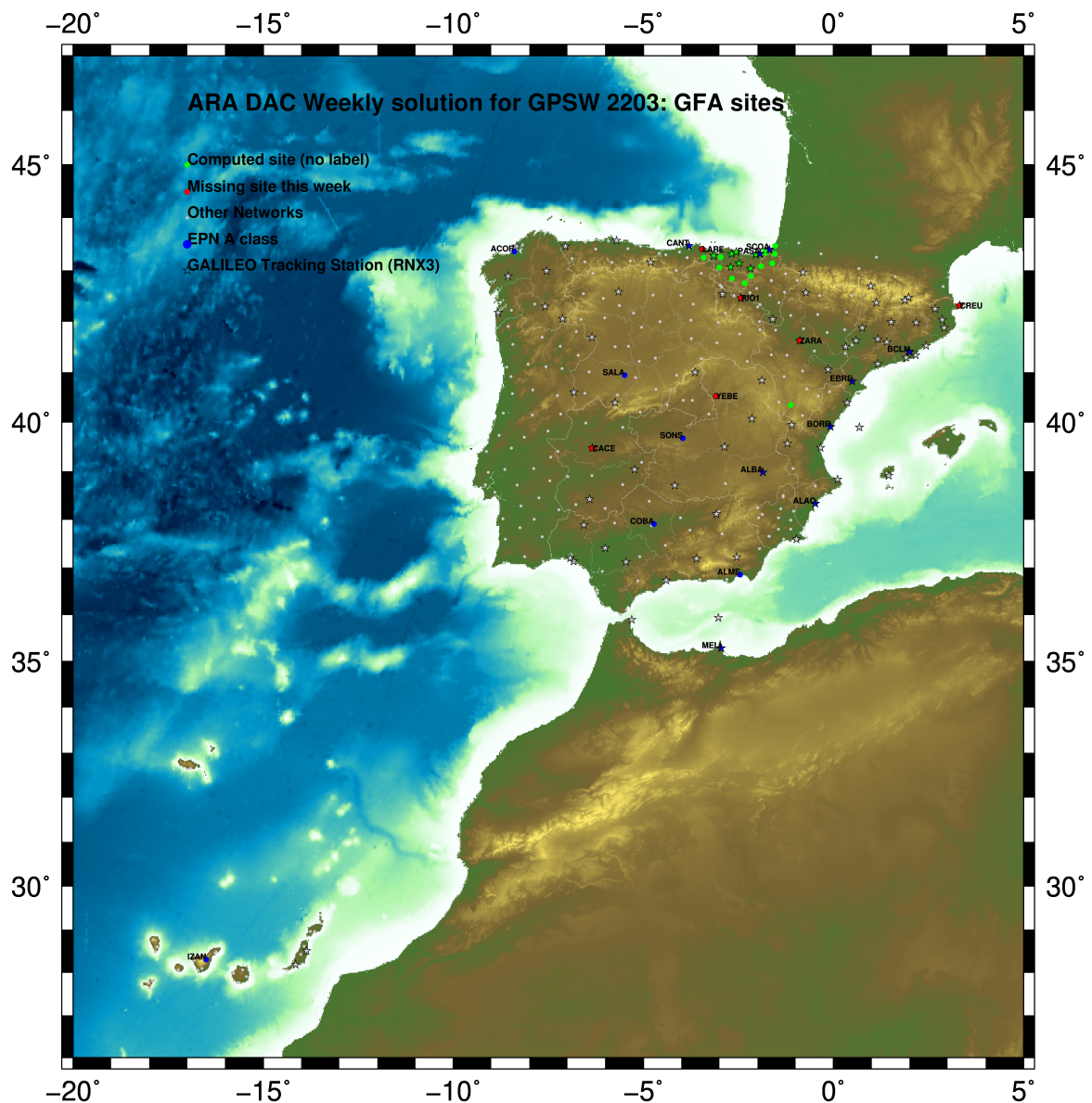
Fig.1: Computed Sites for GPS Week2203 (GFA)
