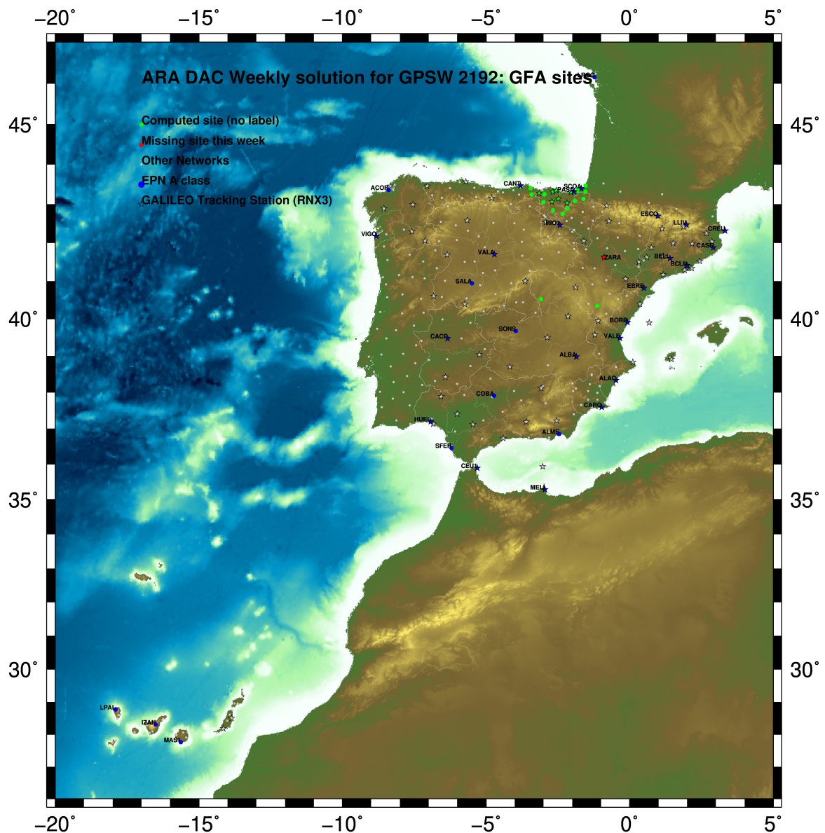
Fig.1: Computed Sites for GPS Week2192 (GFA)
