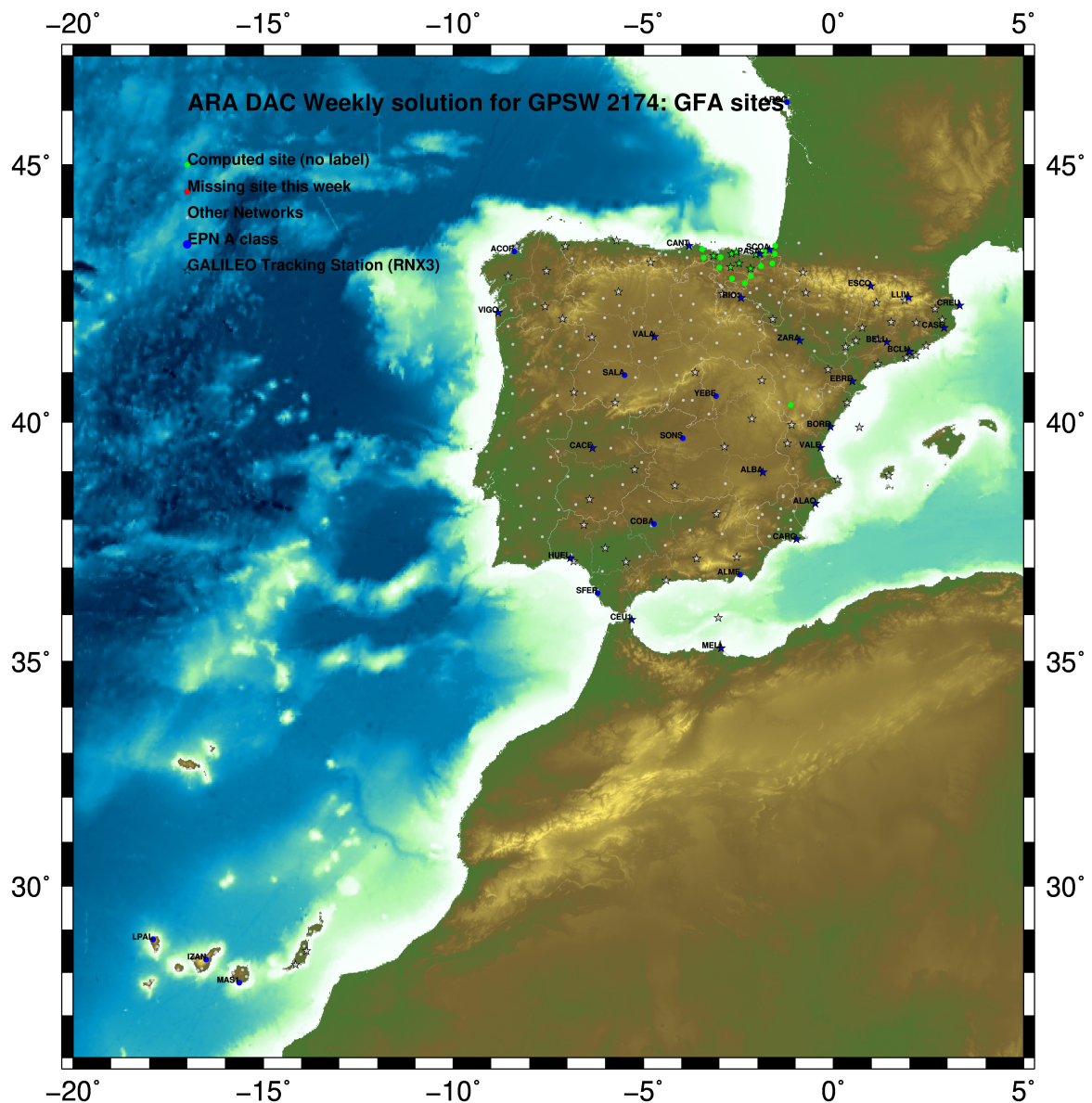
Fig.1: Computed Sites for GPS Week2174 (GFA)
