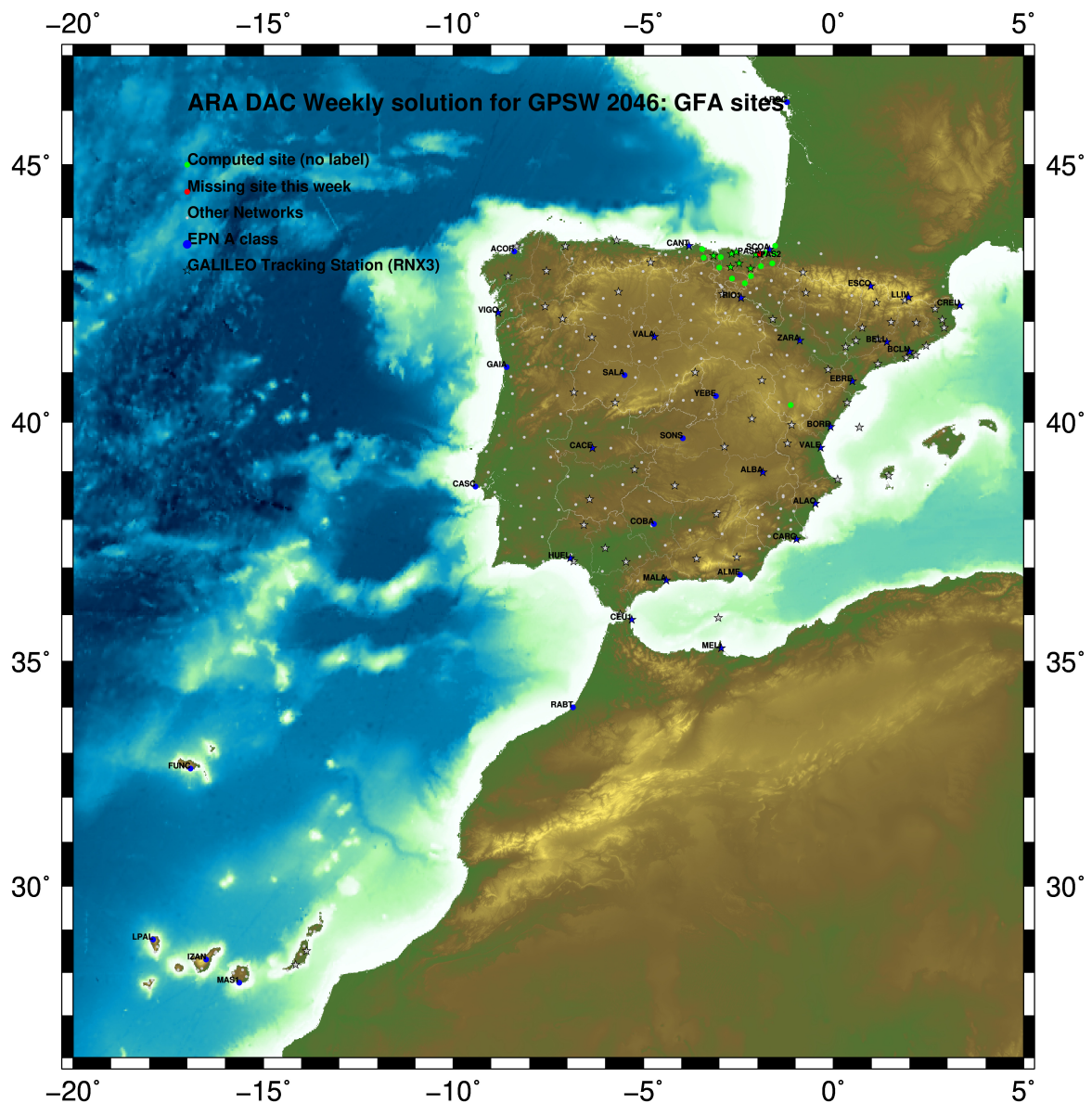
Fig.1: Computed Sites for GPS Week2046 (GFA)
