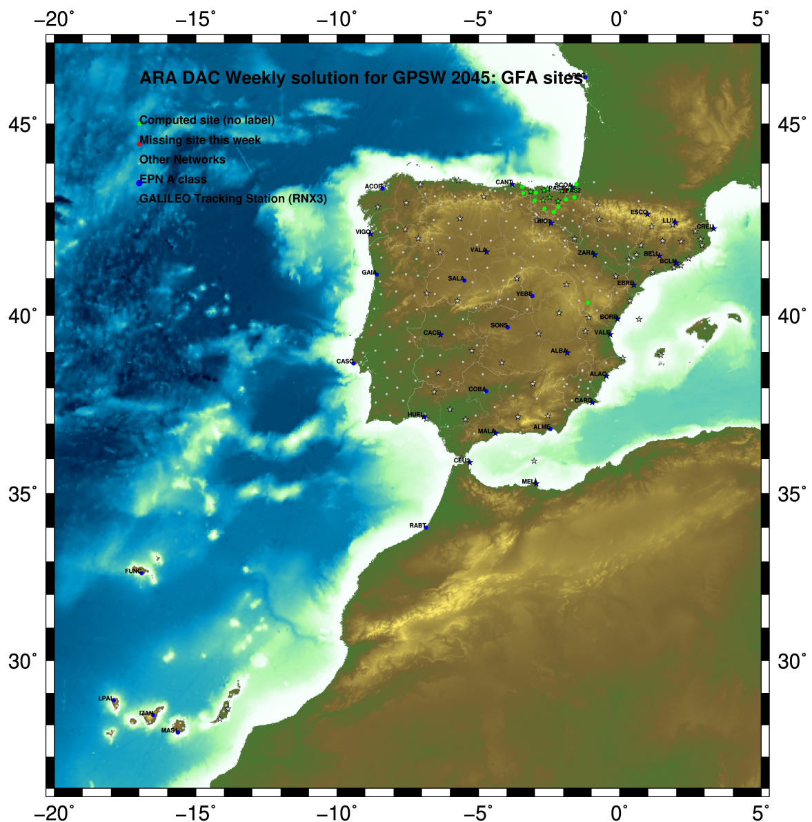
Fig.1: Computed Sites for GPS Week2045 (GFA)
