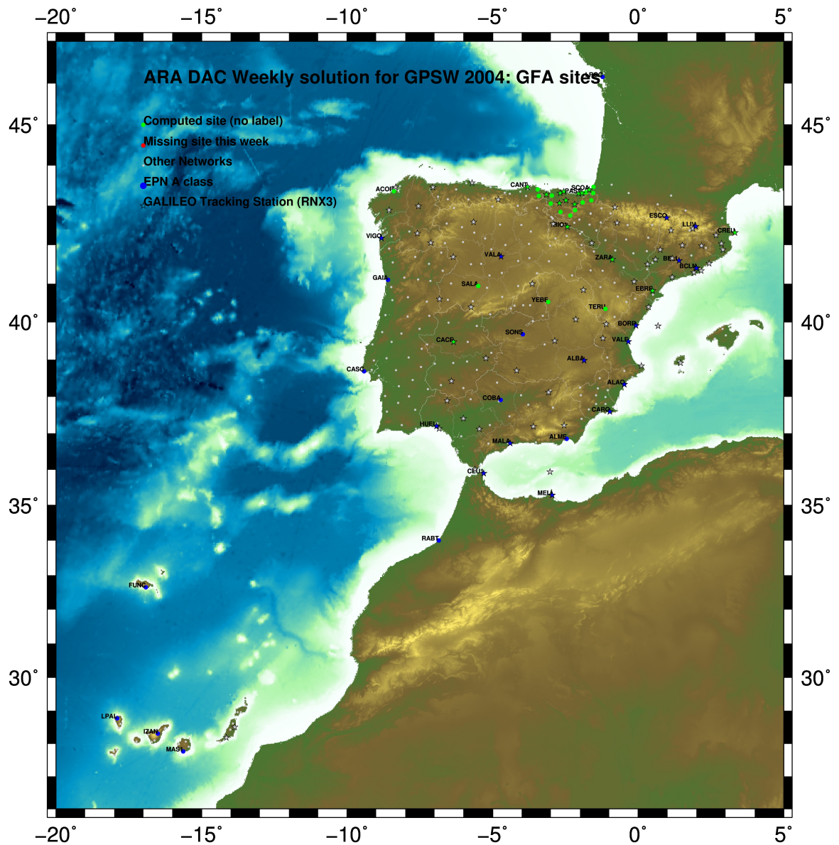
Fig.1: Computed Sites for GPS Week2004 (GFA)
