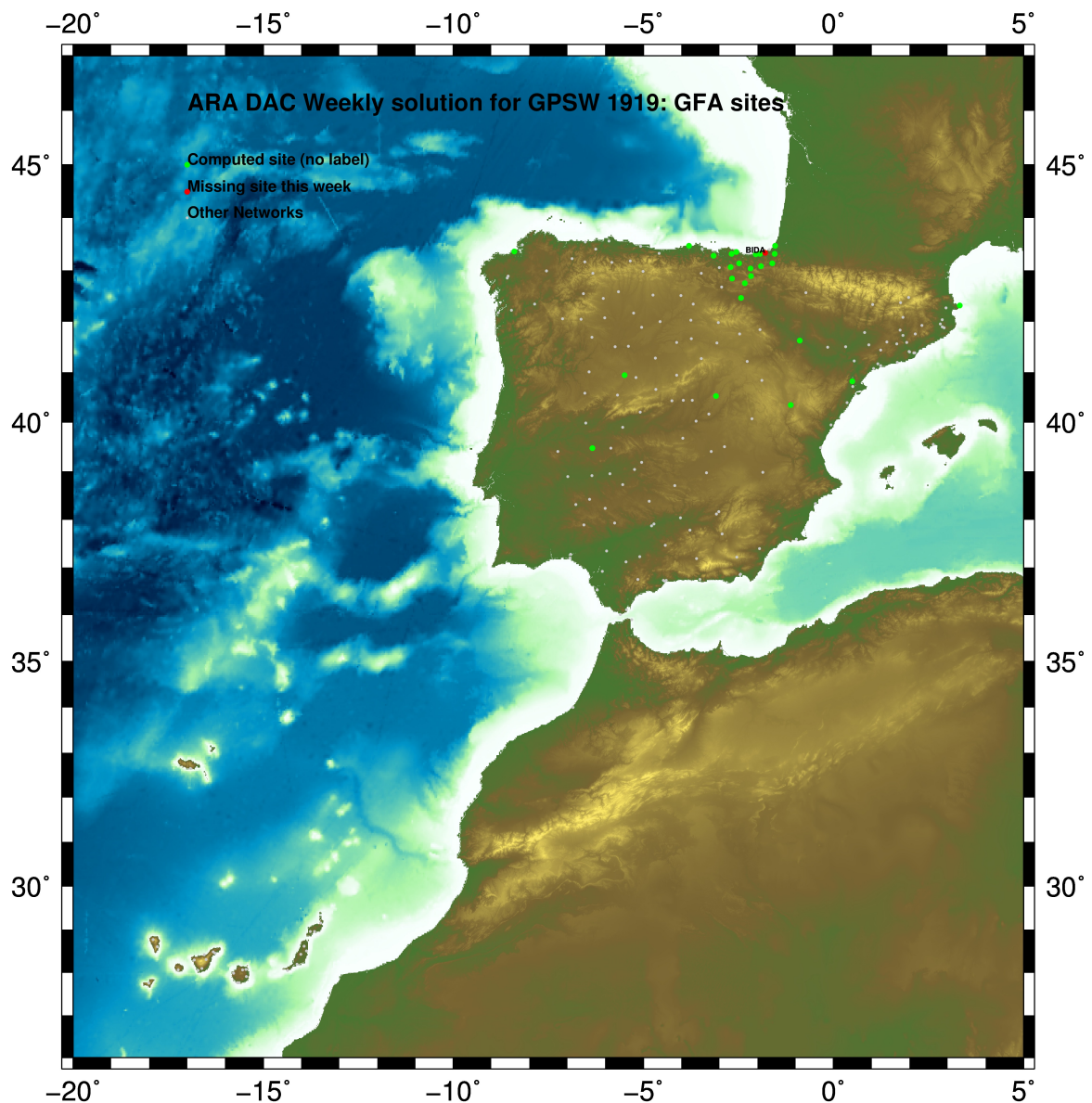
Fig.1: Computed Sites for GPS Week1919 (GFA)
