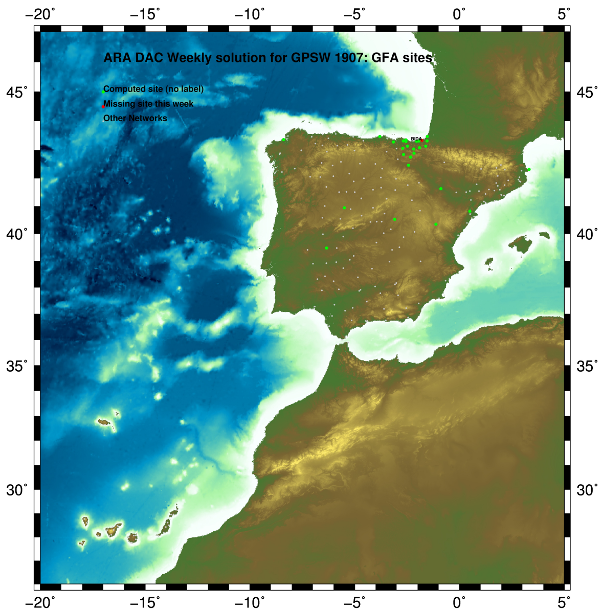
Fig.1: Computed Sites for GPS Week1907 (GFA)
